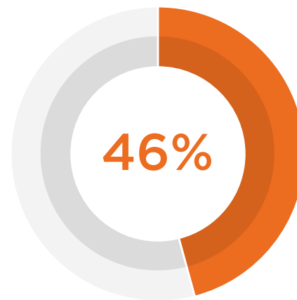
Phishing attack
